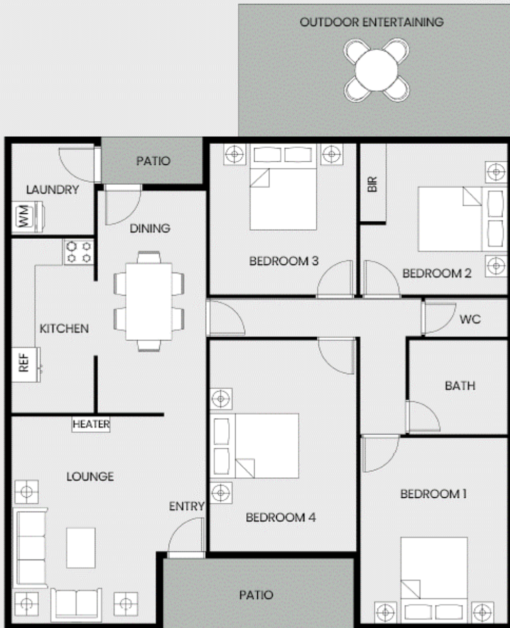
FLOOR PLAN
