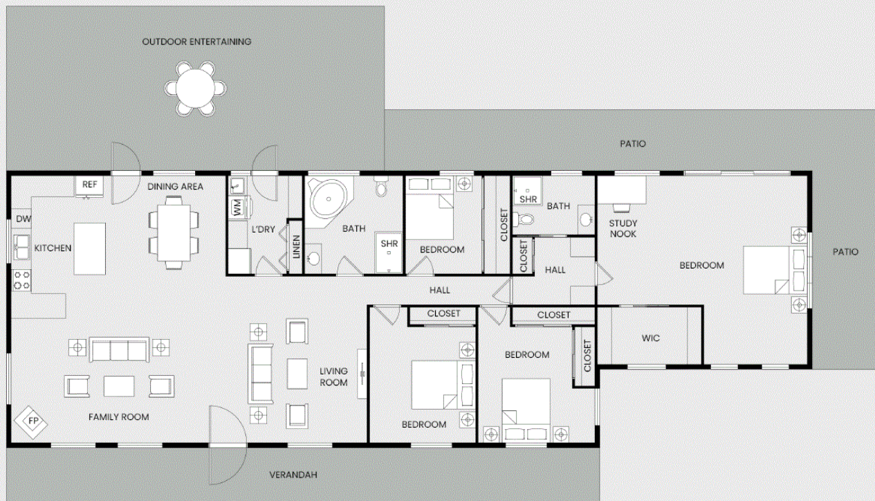
FLOOR PLAN
