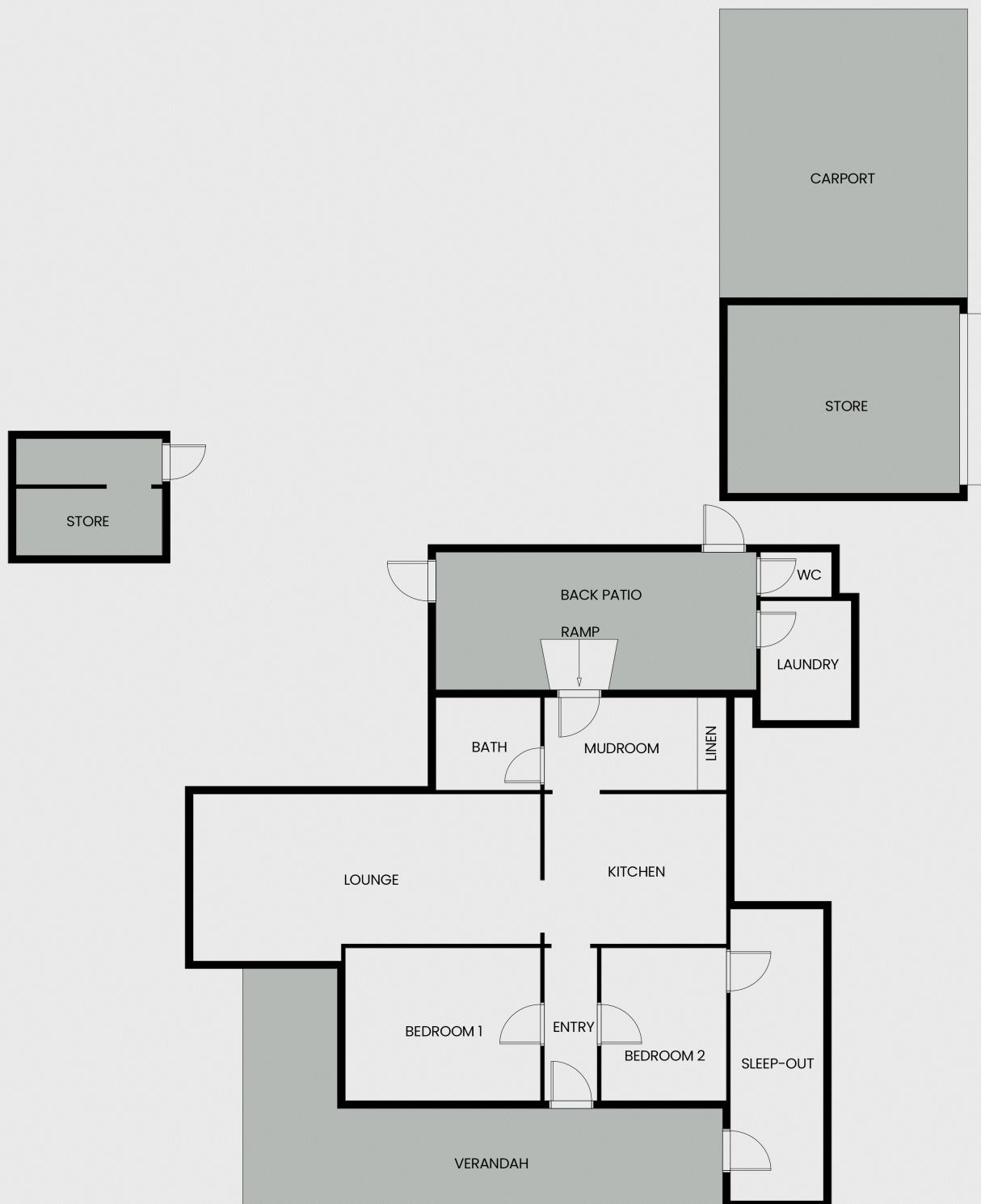
FLOOR PLAN
