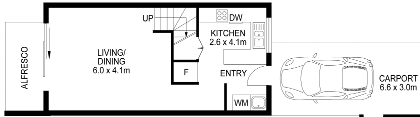
GROUND FLOOR
