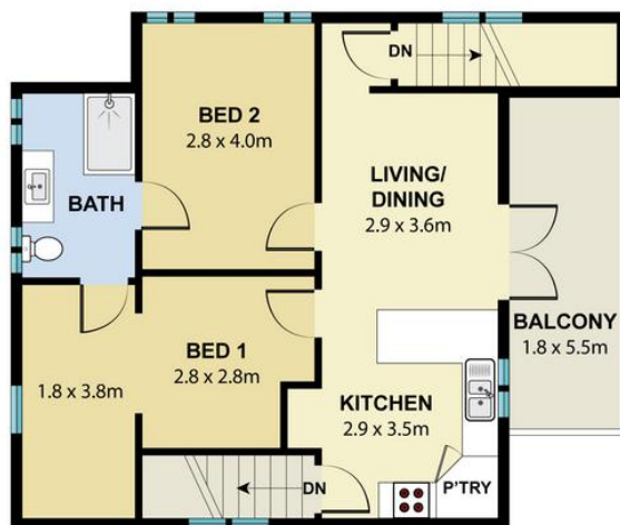
UPPER LEVEL
