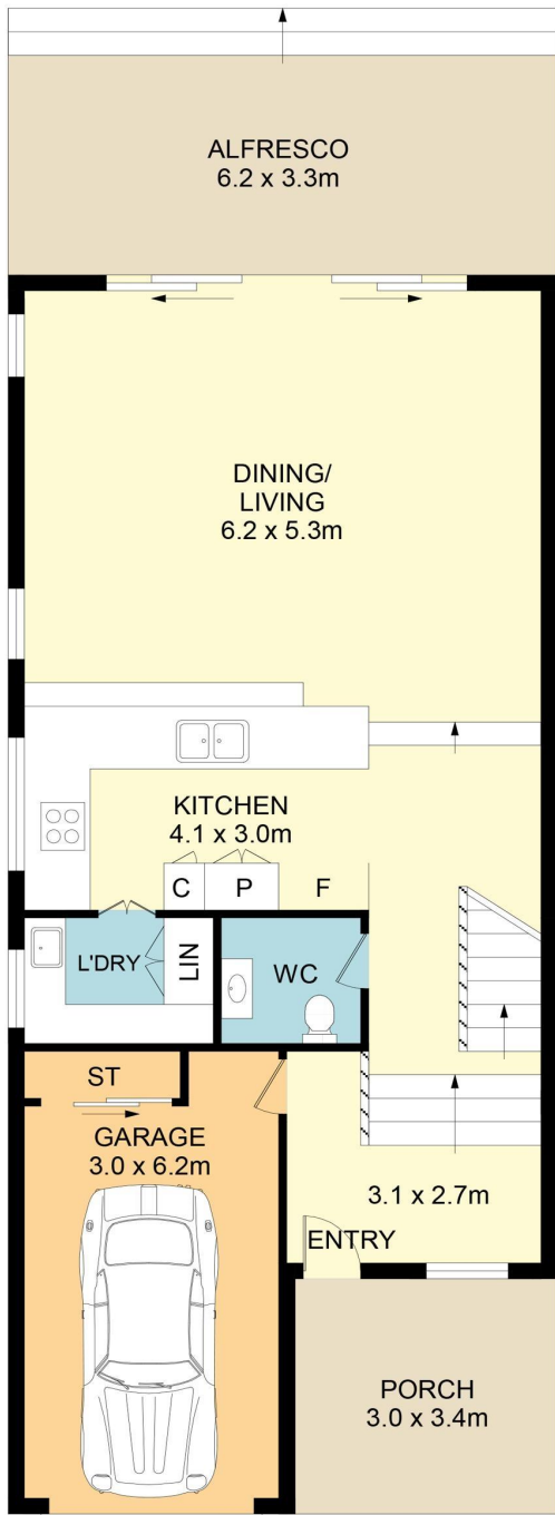
GROUND LEVEL
