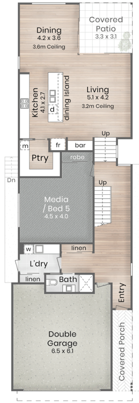
:: FLOOR PLAN Ground Floor - 2.6m Ceiling
