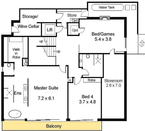
LEVEL 3 Floor Area 200 m2 approx
