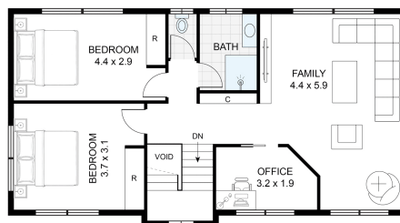
FIRST FLOOR : 82m 2 (EXCLUDES VOID)
