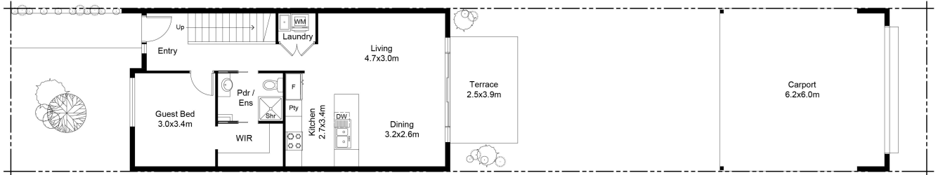
GROUND FLOOR PLAN ON SITE PLAN
