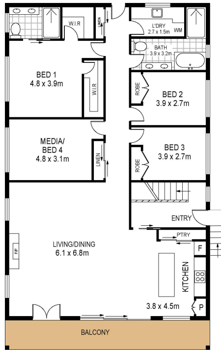
UPPER LEVEL
