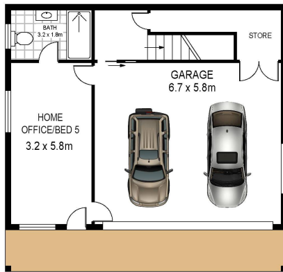
LOWER LEVEL
