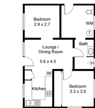
Granny Flat = 48.8 Sq M
