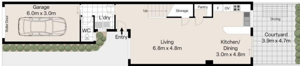
Ground Floor
