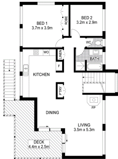
UPPER LEVEL
