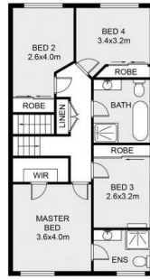
FIRST FLOOR
