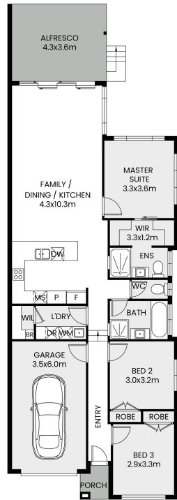
FLOOR PLAN
