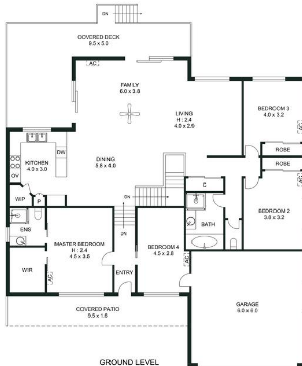
GROUND LEVEL
