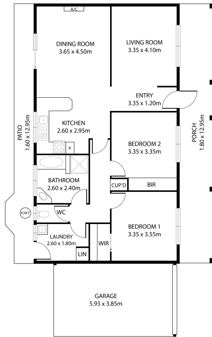
FLOOR PLAN
