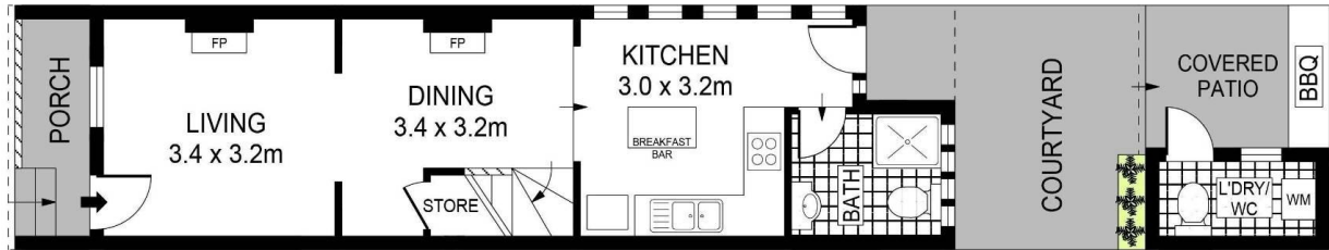
GROUND FLOOR
