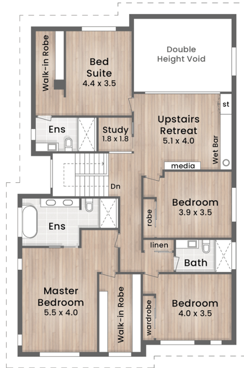
:: FLOOR PLAN First Floor 2.6m Ceiling
