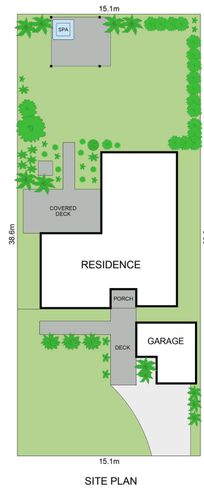
SITE PLAN
