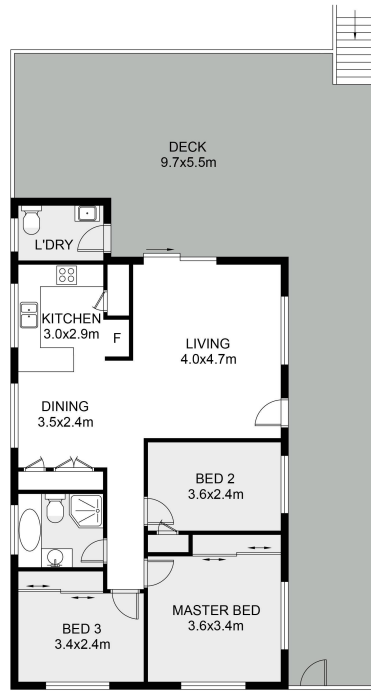
FLOOR PLAN
