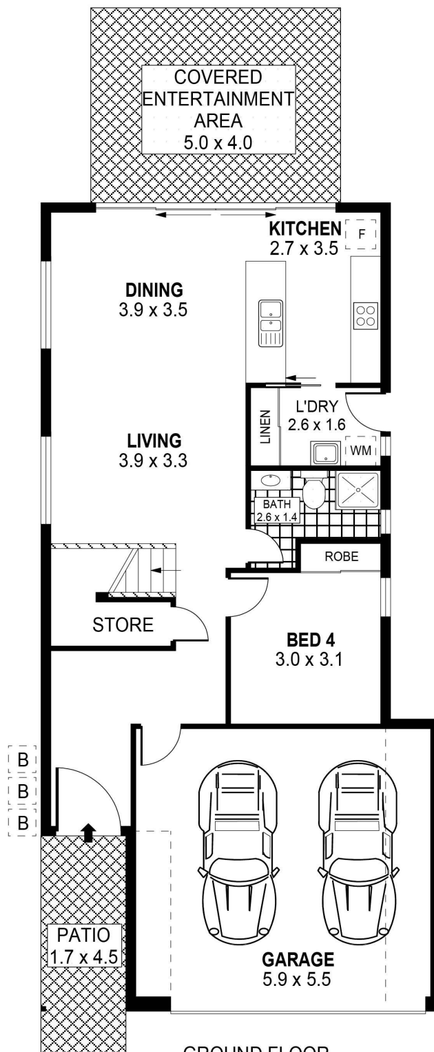
GROUND FLOOR
