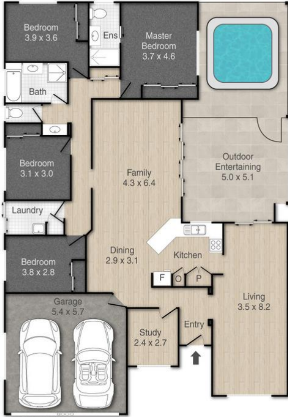
FLOOR PLAN
