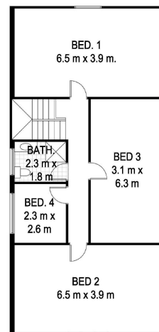
Upper Floor Plan
