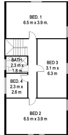
Upper Floor Plan
