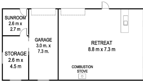
Shed Floor Plan Total Approx. Internal Floor Area: 105 sqm
