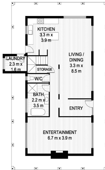
Lower Floor Plan Total Approx. Internal Floor Area: 189 sqm
