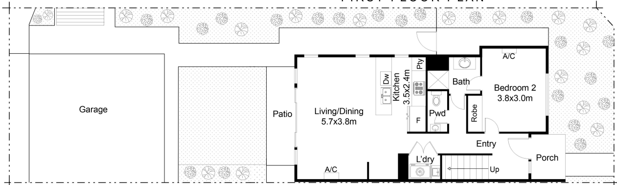
GROUND FLOOR PLAN ON SITE PLAN
