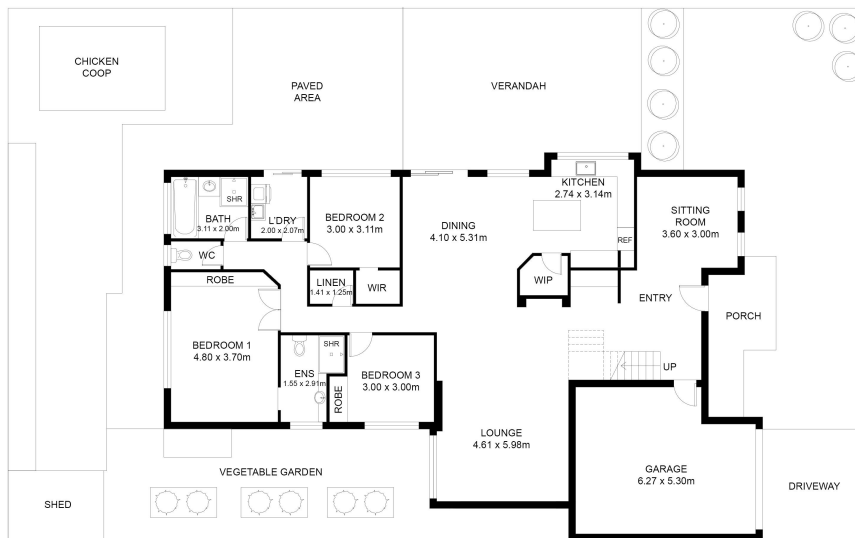
GROUND FLOOR PLAN ON SITE
