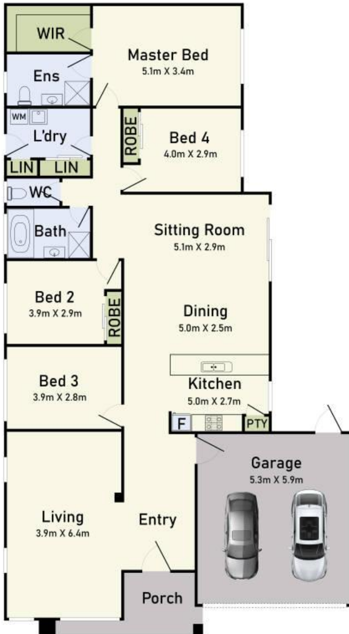
Floor Plan
