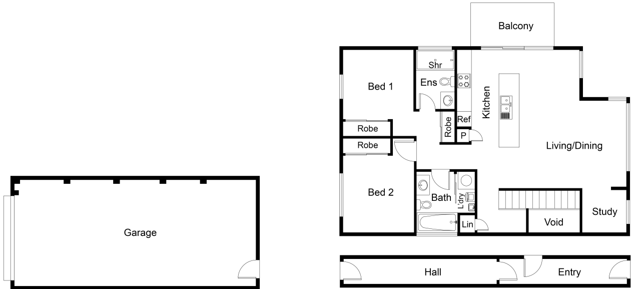
FLOOR PLAN
