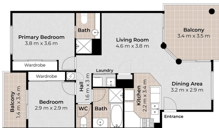
FLOOR PLAN
