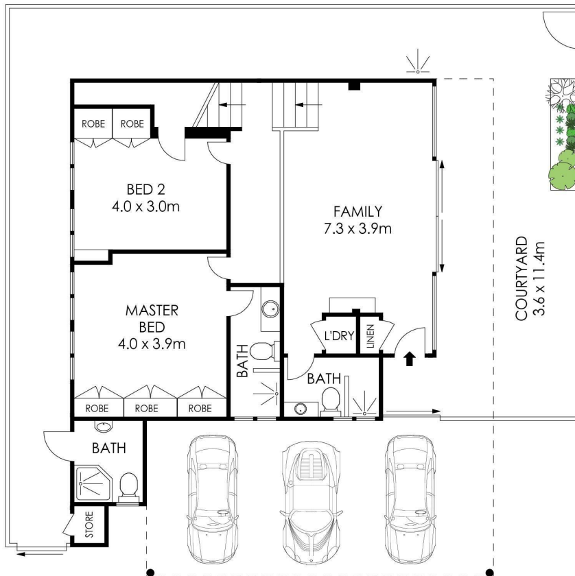
ENTRY LEVEL
