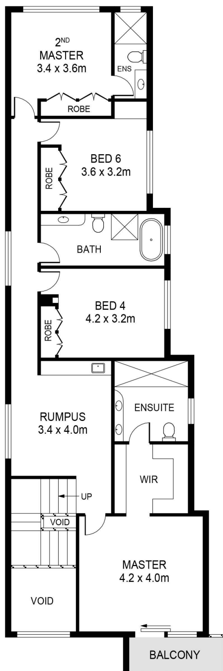
FIRST FLOOR
