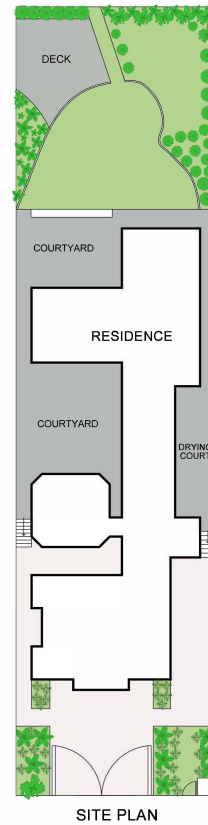
SITE PLAN
