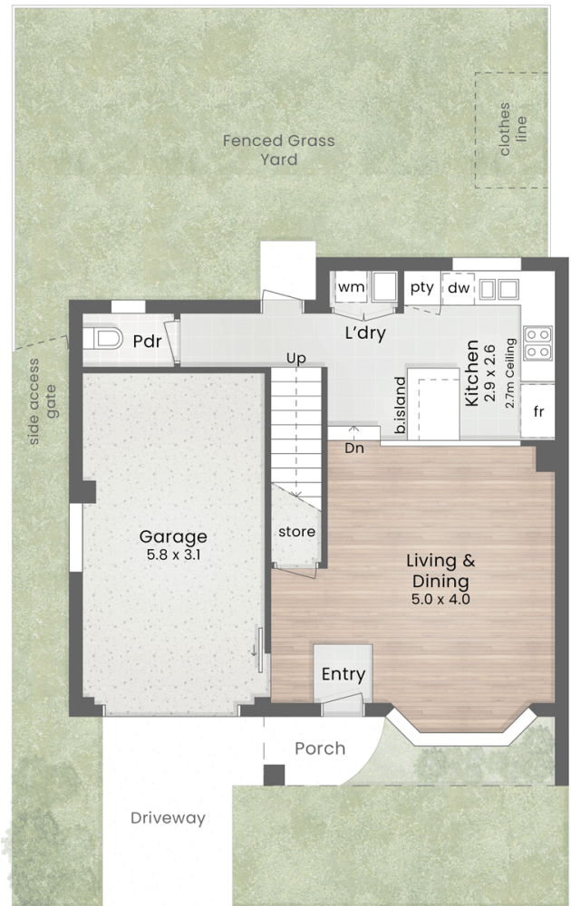
:: GROUND FLOOR PLAN & SITE PLAN DRIVEWAY ACCESS TO CAVENDISH ROAD
