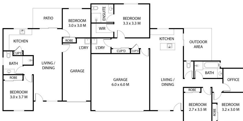
FLOOR PLAN
