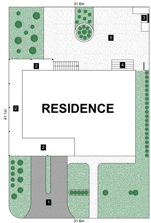
SITE PLAN
