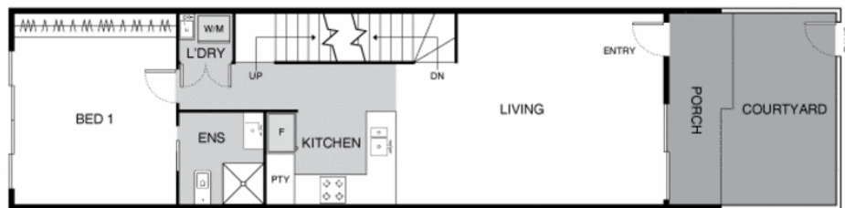
GROUND FLOOR
