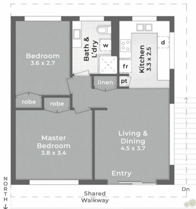
:: FLOOR PLAN Level 1
