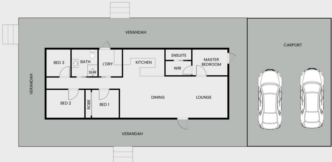
FLOOR PLAN
