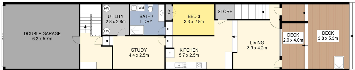
GROUND FLOOR
