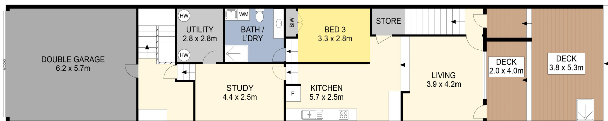
GROUND FLOOR
