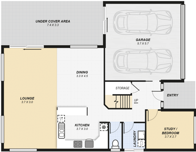
GROUND LEVEL
