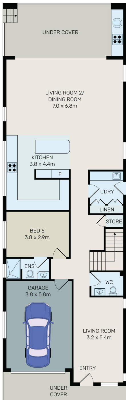
GROUND FLOOR
