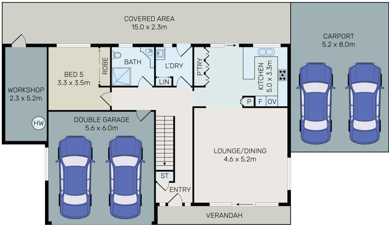
GROUND FLOOR
