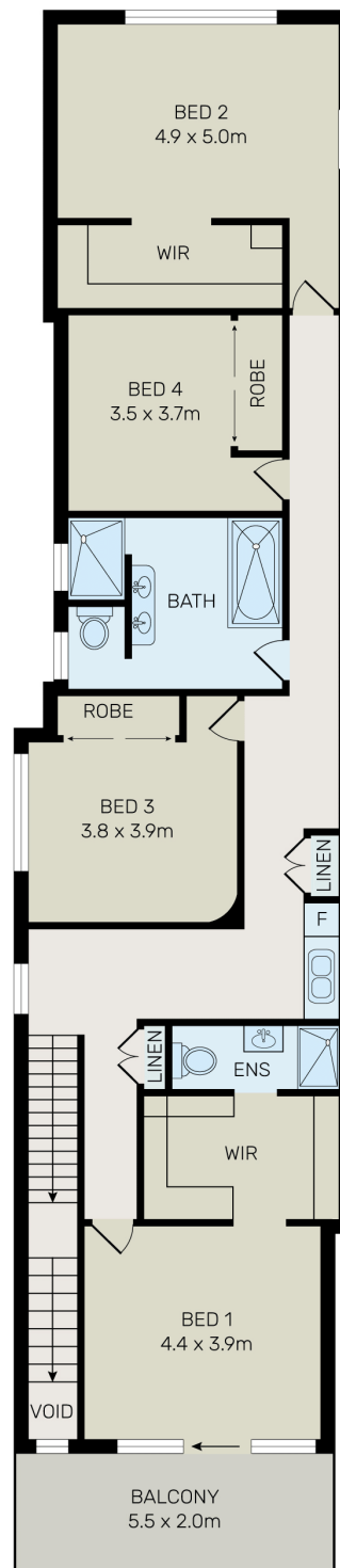
FIRST FLOOR
