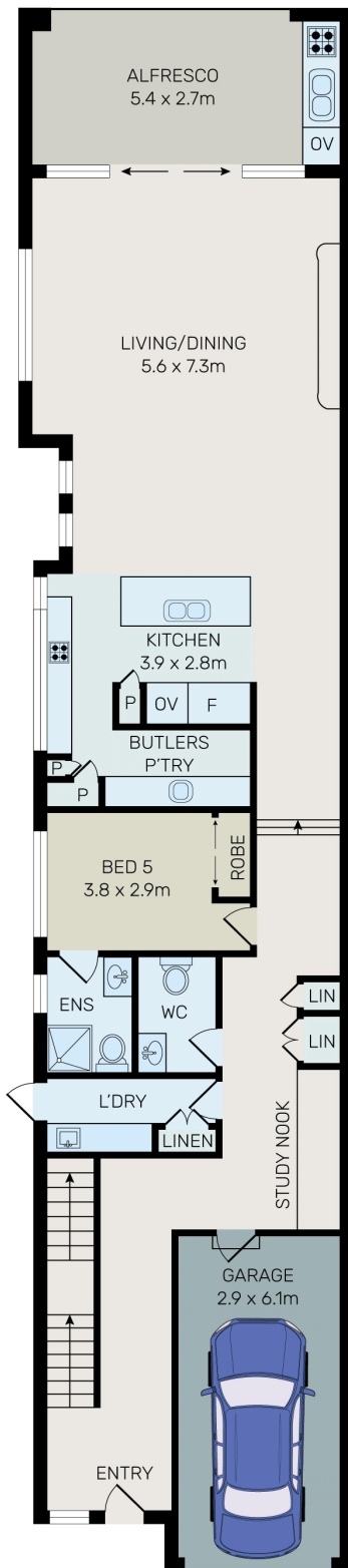
GROUND FLOOR
