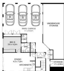
GROUND FLOOR
