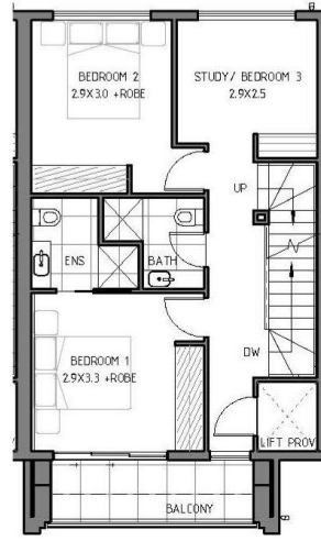
Level 2 Floor Plan
