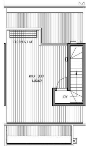
Level 3 Floor Plan
