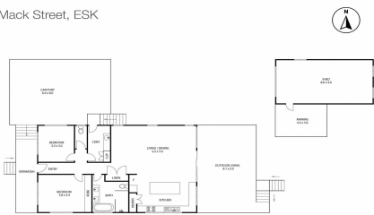
This floor plan illustration is an approximation of existing structures and features and is provided for convenience only with the permission of the seller. All measurements and mtl are approximate and not guaranteed to be exact or to scale. Buyer should confirm measurements using their own source. Bedrooms are measured from wall to robe.
