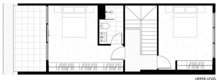
UPPER LEVEL
